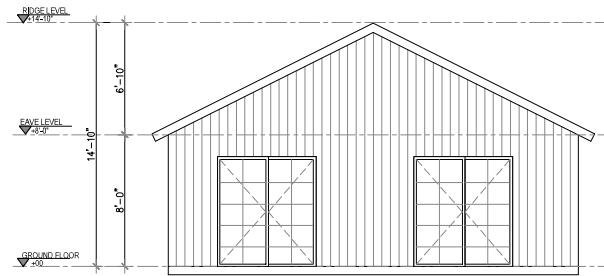
1 FRONT ELEVATION Scale 1'=1/8"
