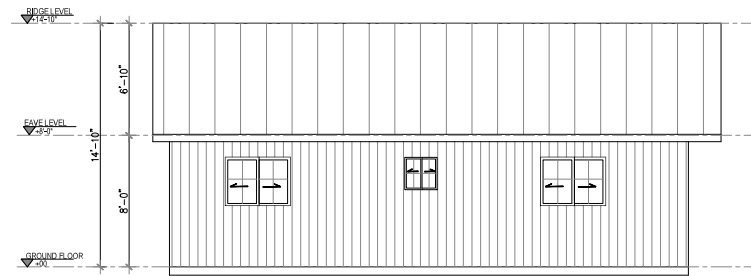
4 LEFT SIDE ELEVATION Scale 1'=1/8"
