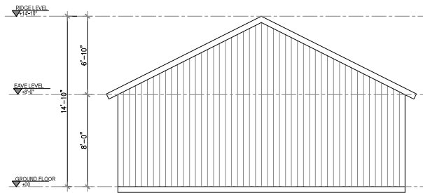
2 REAR ELEVATION Scale 1'=1/8"
