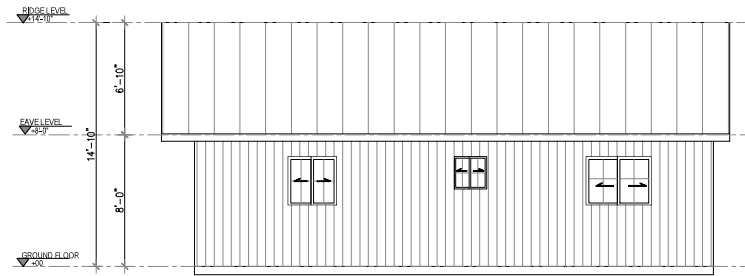
3 RIGHT SIDE ELEVATION Scale 1'=1/8"
