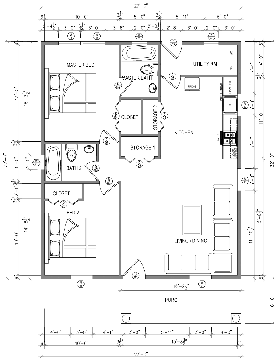
1 GROUND FLOOR PLAN Scale 1"=3/16"
