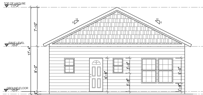
2 REAR ELEVATION Scale 1"=1/8"
