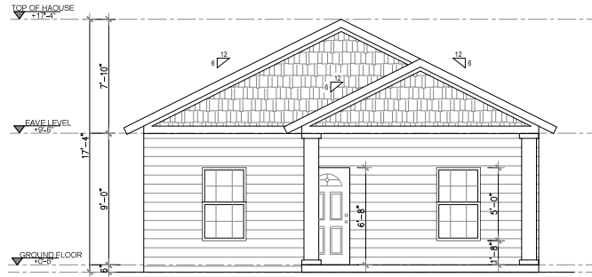
1 FRONT ELEVATION Scale 1"=1/8"
