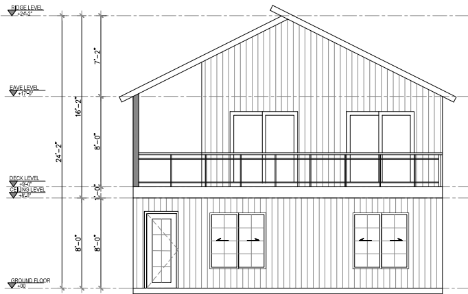
1 FRONT ELEVATION Scale 1"=1/8"
