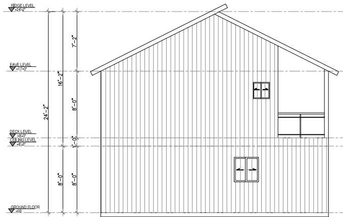
2 REAR ELEVATION Scale 1"=1/8"
