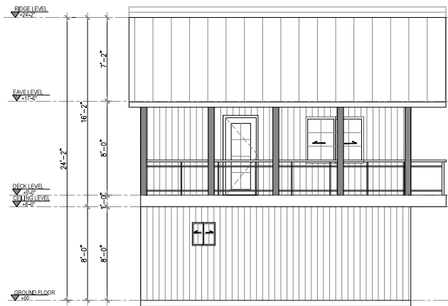
3 LEFT SIDE ELEVATION Scale 1"=1/8"
