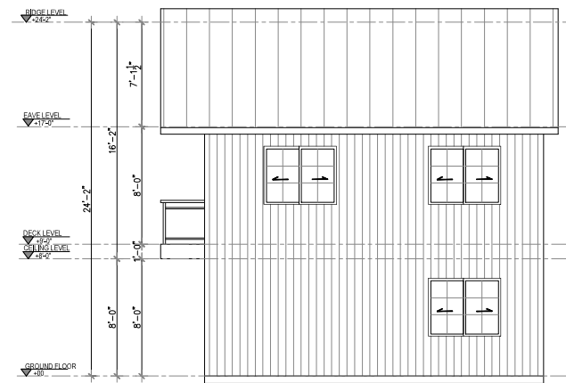
4 RIGHT SIDE ELEVATION Scale 1"=1/8"
