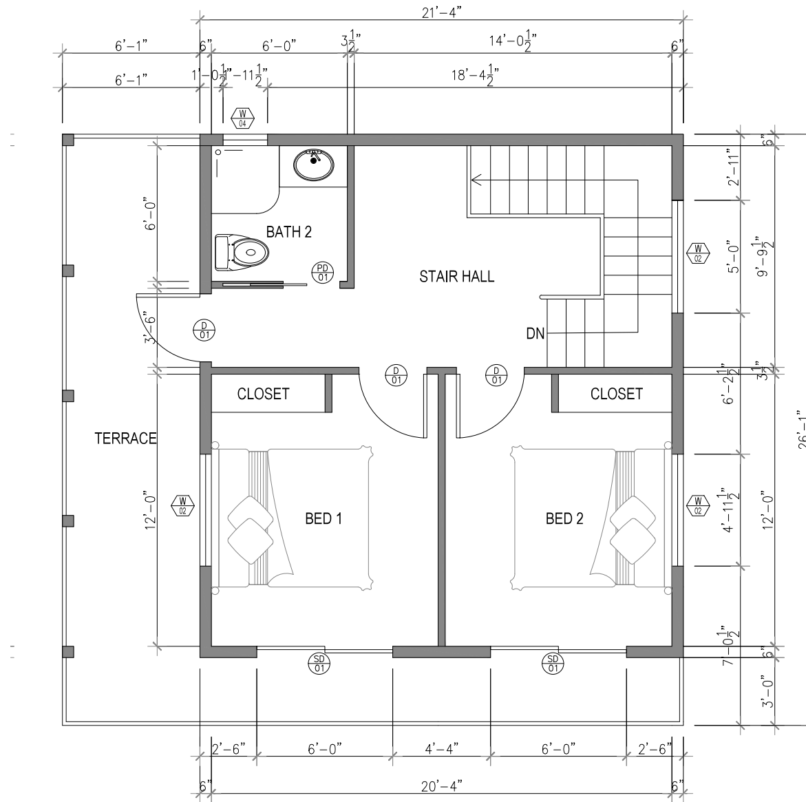
1 FIRST FLOOR PLAN Scale 1"=1/4"
