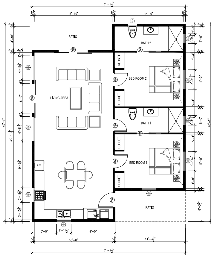
1 GROUND FLOOR PLAN Scale 1"=1/8"
