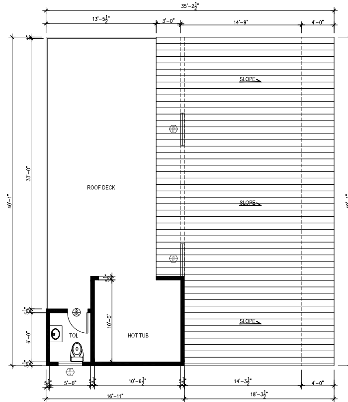
2 ROOF FLOOR PLAN Scale 1"=1/8"
