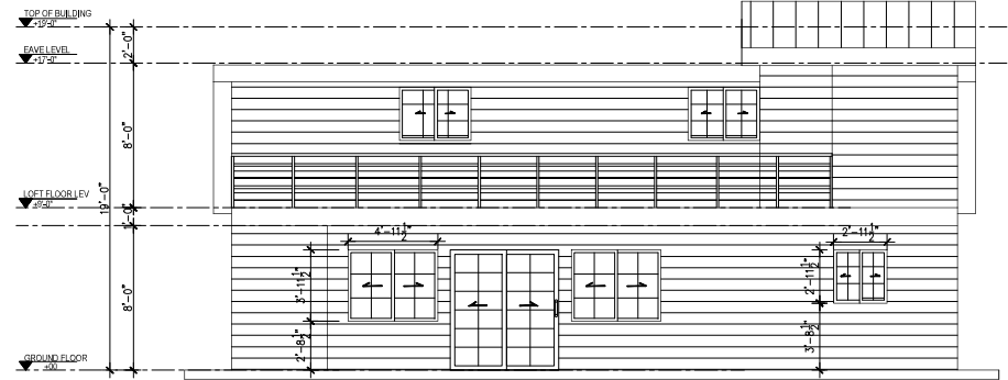
4 LEFT SIDE ELEVATION Scale 1=1/8"
