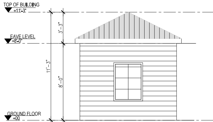
4 LEFT SIDE ELEVATION Scale 1"=1/4"
