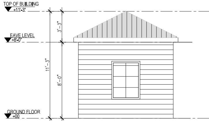
3 RIGHT SIDE ELEVATION Scale 1"=1/4"
