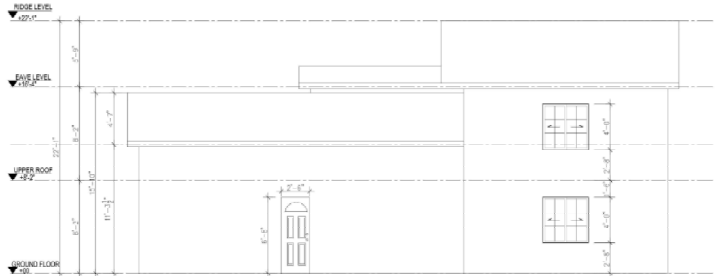
2 BACK ELEVATION Scale 1"=1/8"
