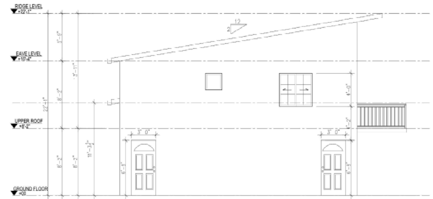
3 RIGHT ELEVATION Scale 1"=1/4"
