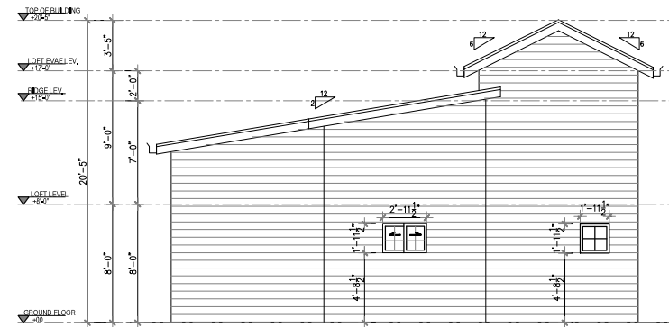
2 REAR ELEVATION Scale 1"=14"
