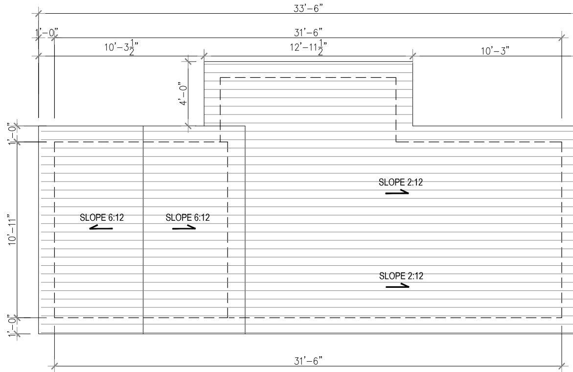
1 ROOF FLOOR PLAN Scale 1'=1/4"
