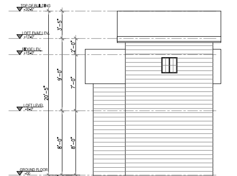
4 LEFT ELEVATION Scale 1"=14"
