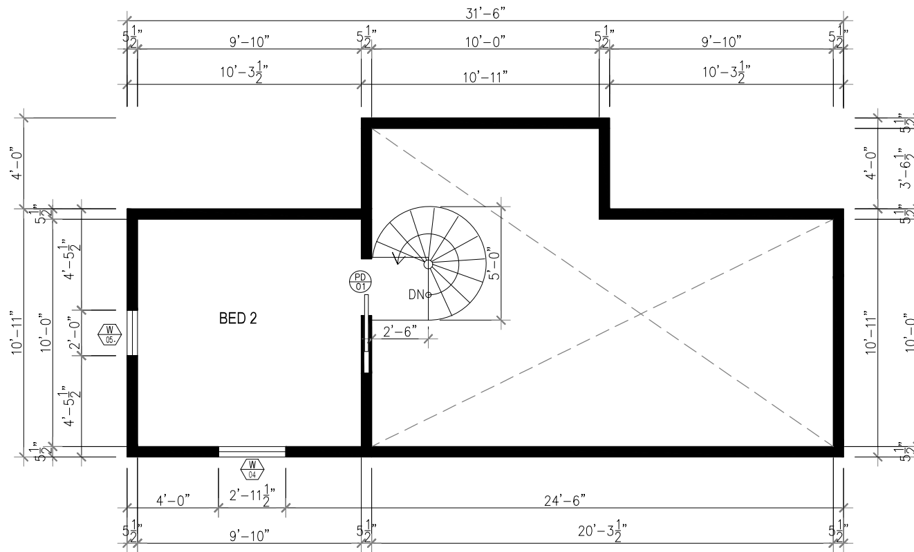
1 LOFT FLOOR PLAN Scale 1"=1/4"
