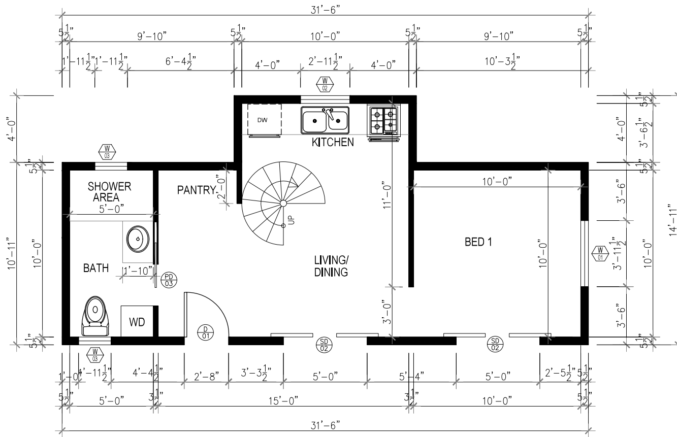
1 GROUND FLOOR PLAN Scale 1"=1/4"
