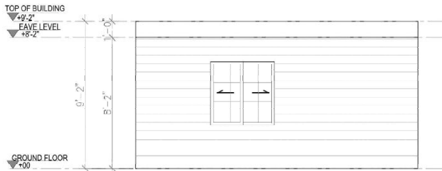
2 REAR ELEVATION Scale 1'=1/4"
