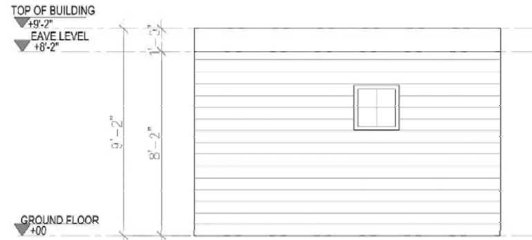
3 RIGHT SIDE ELEVATION Scale 1'=1/4"
