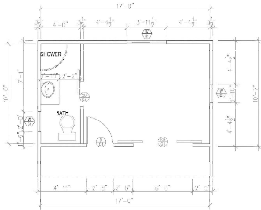
1 GROUND FLOOR PLAN Scale 1"=1/4"
