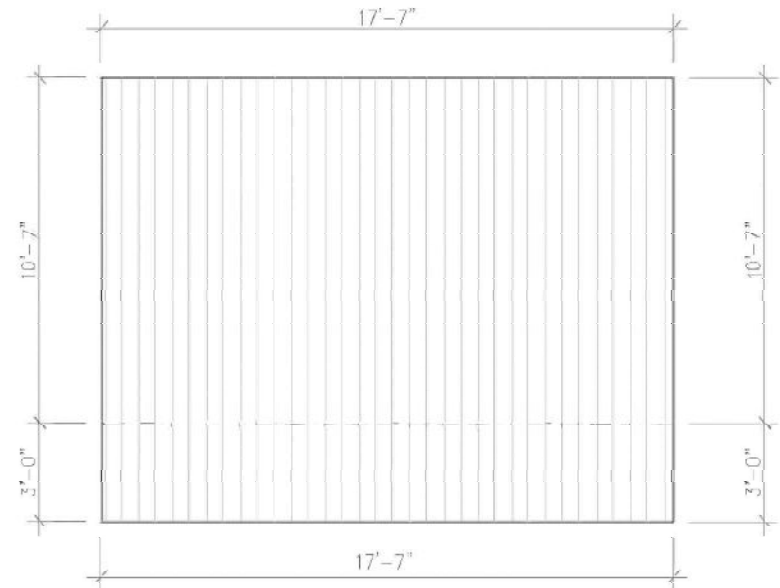
2 ROOF FLOOR PLAN Scale 1"=1/4"
