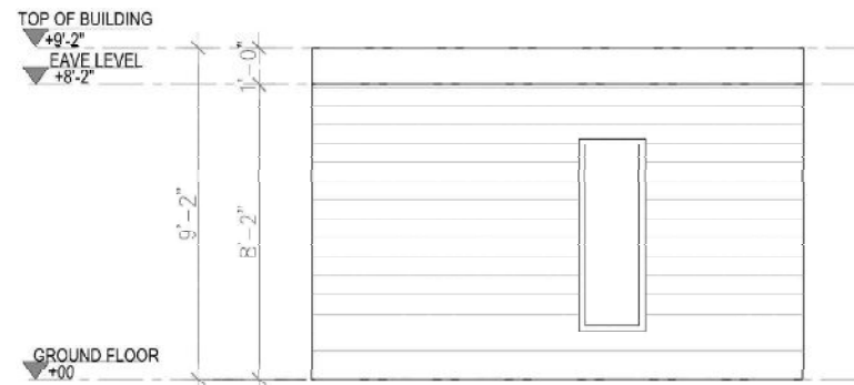
4 LEFT SIDE ELEVATION Scale 1'=1/4"
