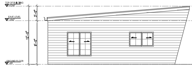
3 RIGHT ELEVATION Scale: 1"=1/4"
