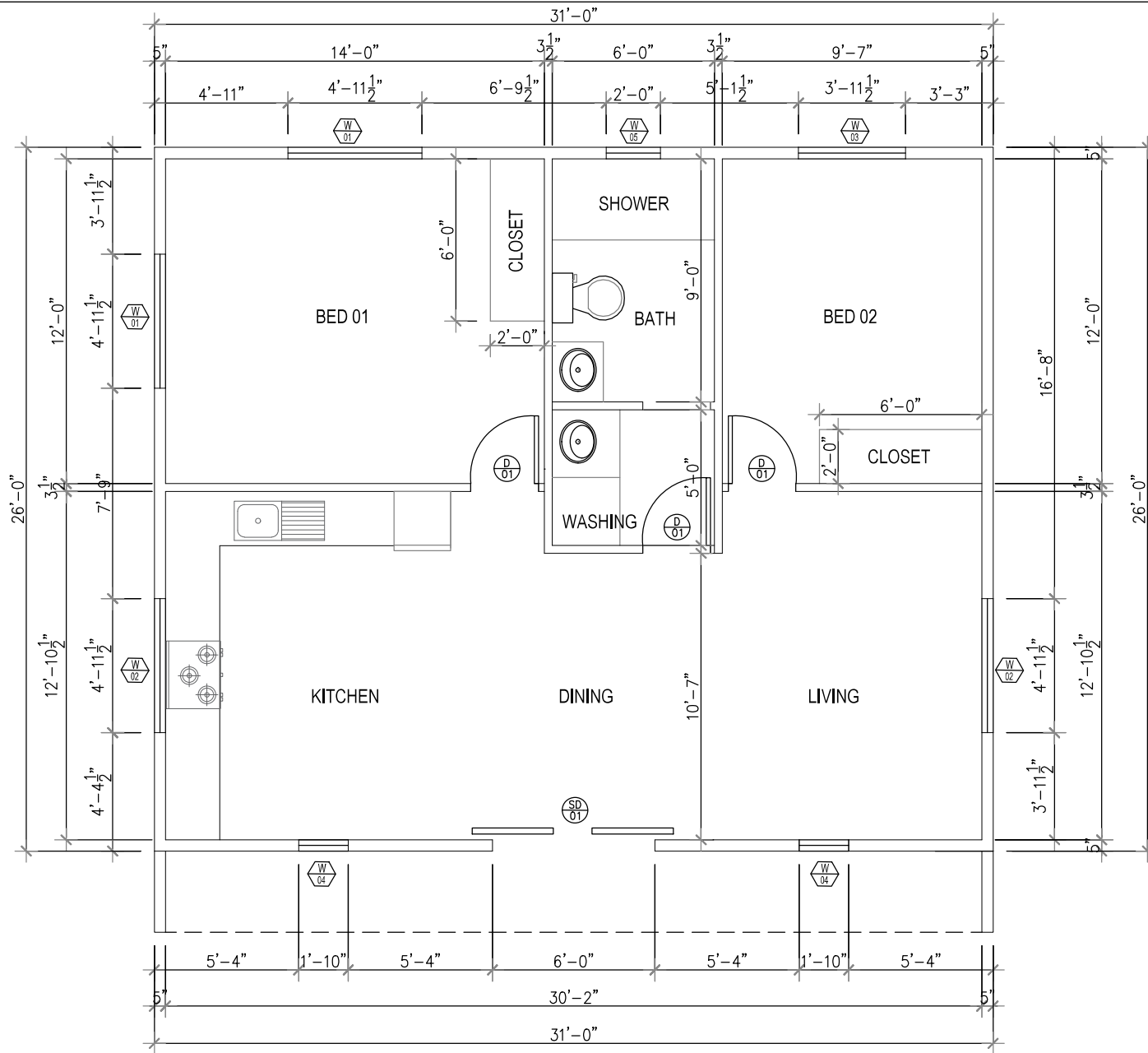
1 GROUND FLOOR PLAN Scale 1/4"
