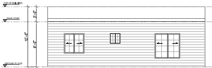
2 REAR ELEVATION Scale: 1"=1/4"
