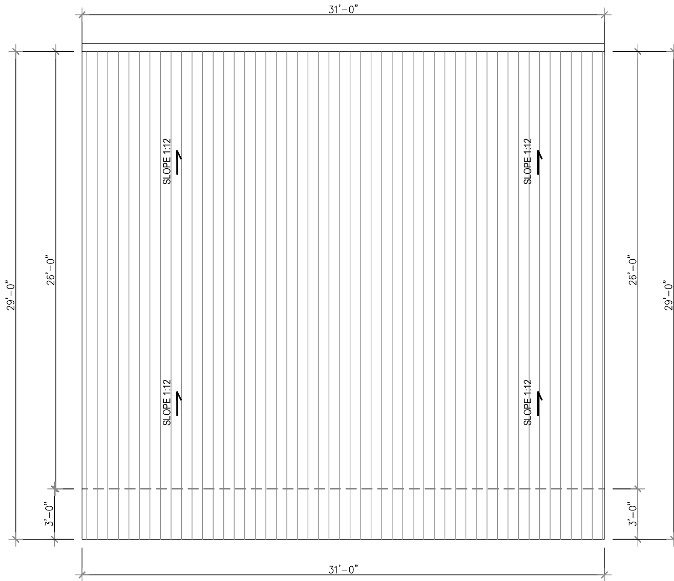
1 ROOF FLOOR PLAN Scale 1"=1/4"
