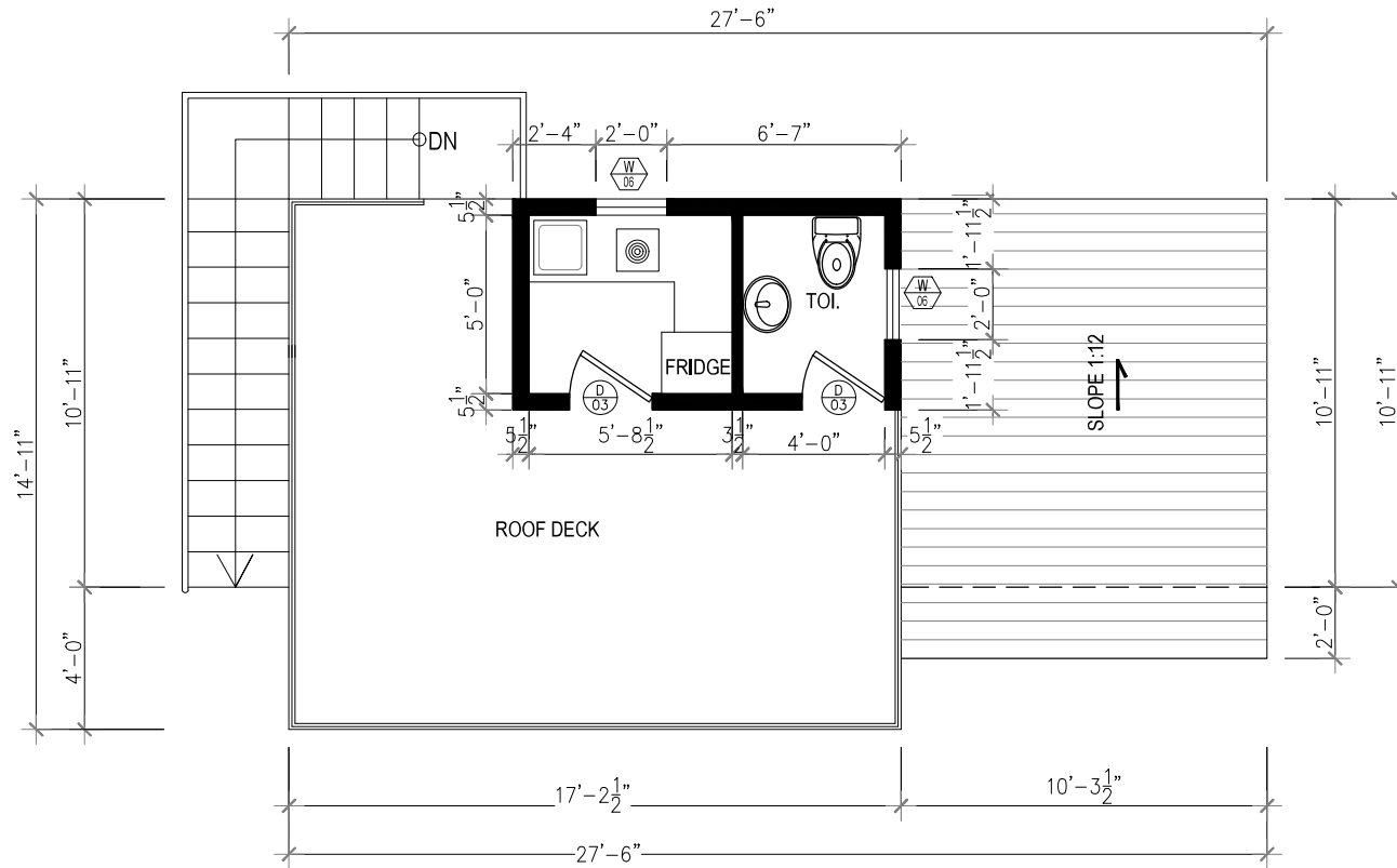
1 ROOF FLOOR PLAN Scale 1"=1/4"
