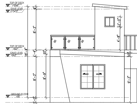
4 LEFT ELEVATION Scale 1"=1/8"
