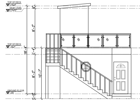
3 RIGHT ELEVATION Scale 1"=1/8"
