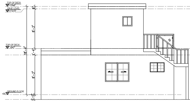
2 REAR ELEVATION Scale 1"=1/8"
