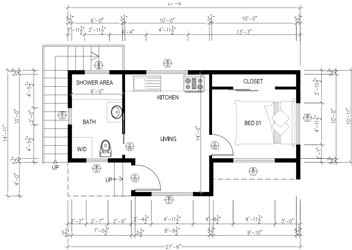
1 GROUND FLOOR PLAN Scale 1"=1/4"
