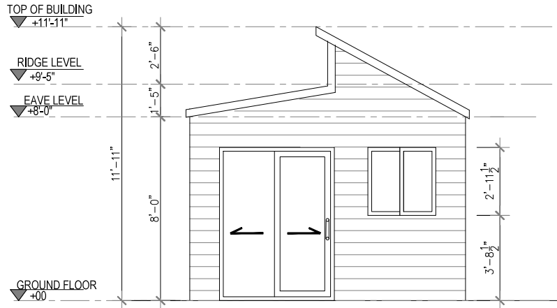
1 FRONT ELEVATION Scale 1"=1/4"
