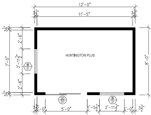
1 GROUND FLOOR PLAN Scale 1"=1/4"
