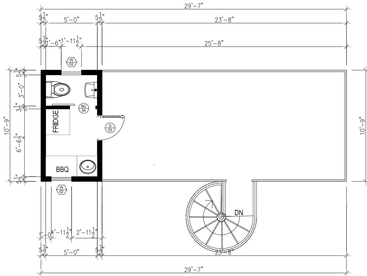
1 ROOF FLOOR PLAN SCALE= 1'=1/4"
