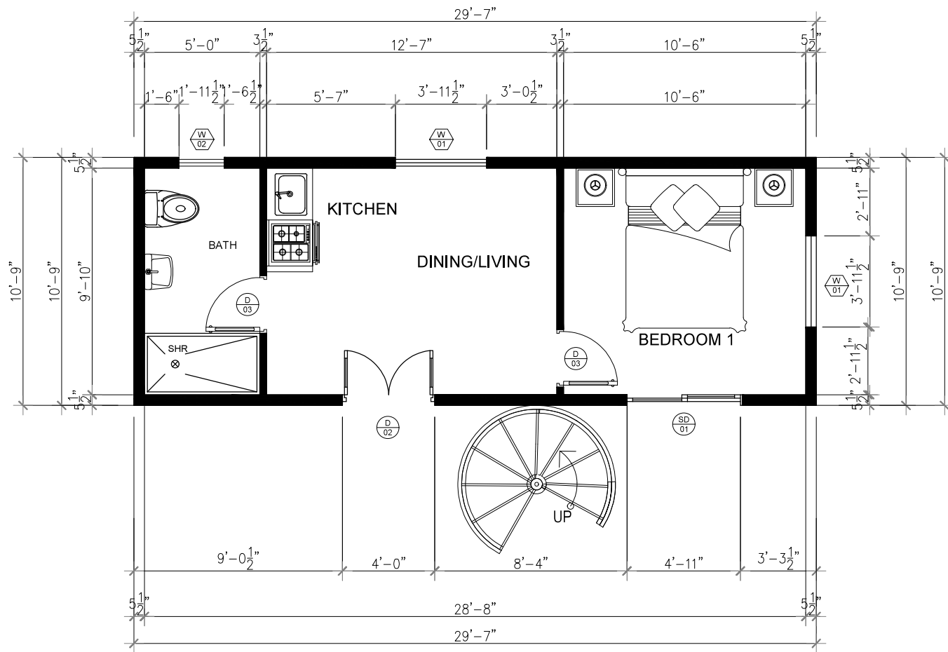
1 GROUND FLOOR PLAN SCALE= 1"=1/4"
