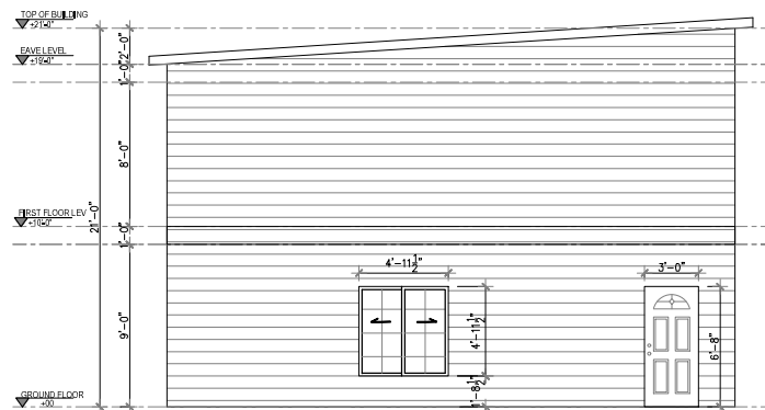
4 LEFT SIDE ELEVATION Scale 1=1/4
