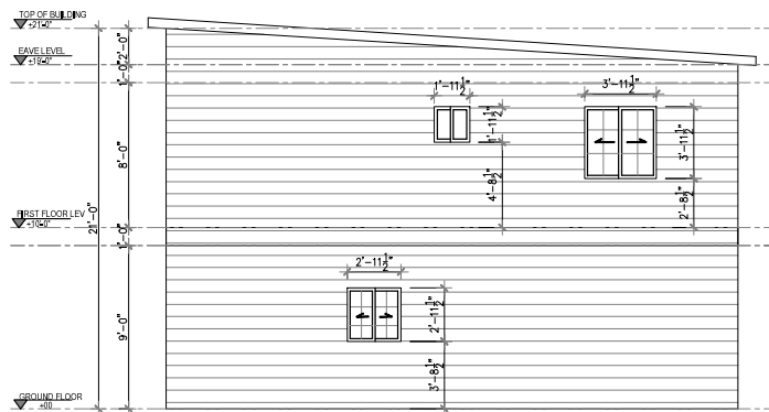
3 RIGHT SIDE ELEVATION Scale 1=1/4
