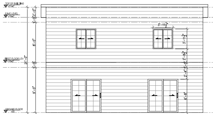
1 FRONT ELEVATION Scale 1=1/4
