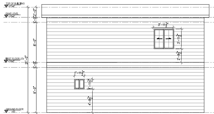
2 REAR ELEVATION Scale 1=1/4
