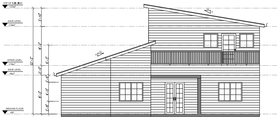
1 FRONT ELEVATION Scale 1"=1/8"
