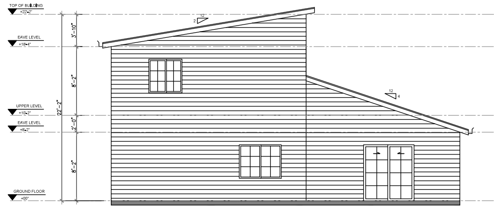
2 REAR ELEVATION Scale 1"=1/8"
