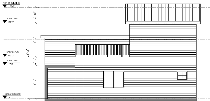
3 RIGHT SIDE ELEVATION Scale 1"=1/8"
