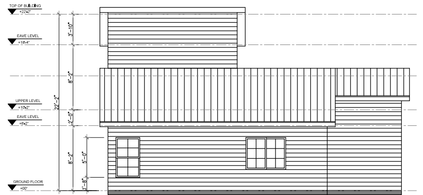
4 LEFT SIDE ELEVATION Scale 1"=1/8"
