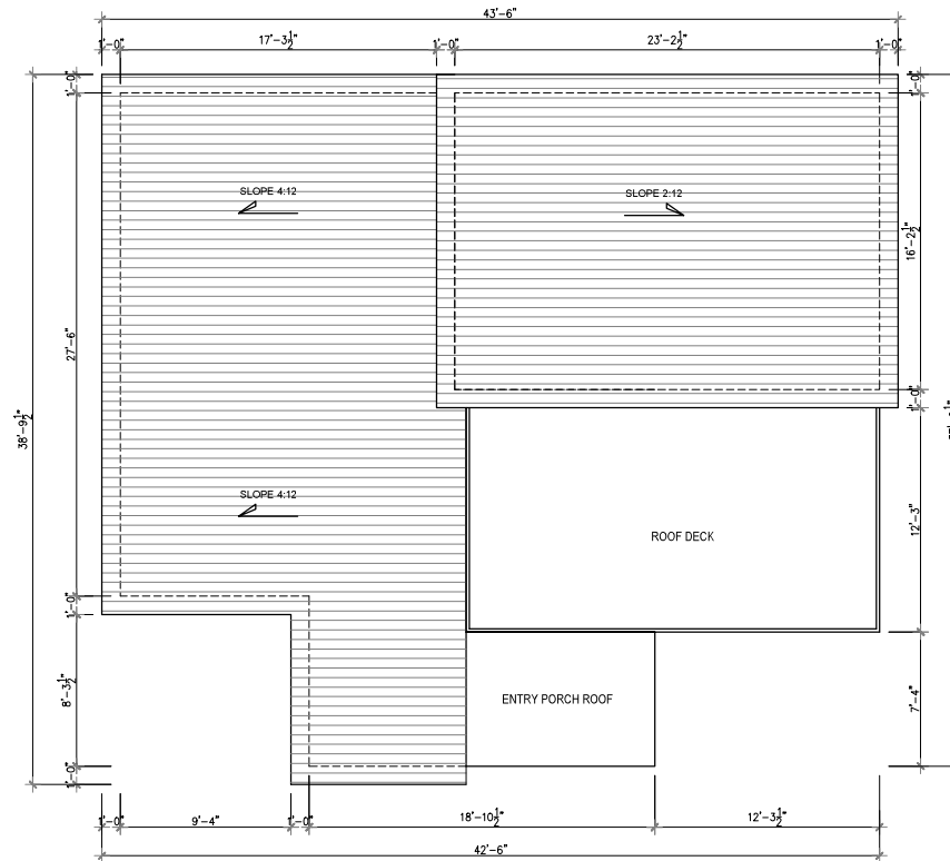
1 ROOF FLOOR PLAN Scale: 1"=1/8"
