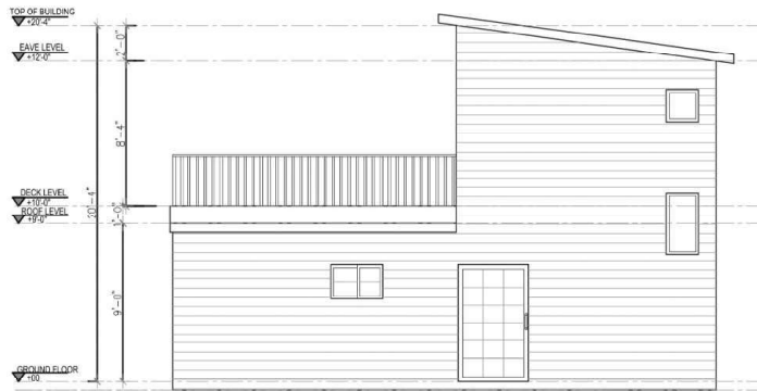
1 FRONT ELEVATION Scale 1"=18"
