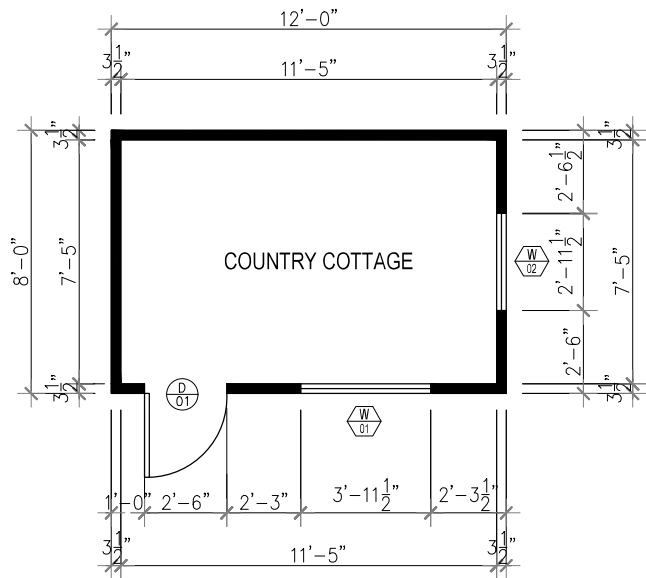
1 GROUND FLOOR PLAN Scale 1'=1/4"
