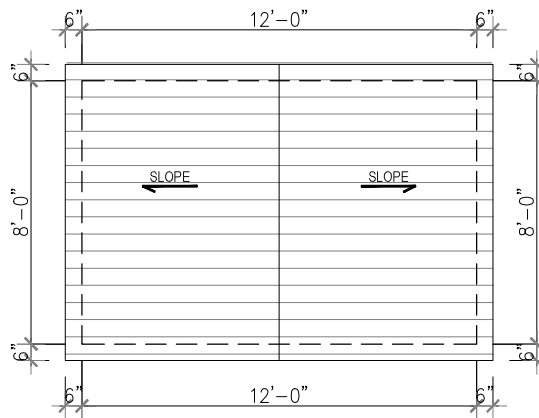
2 ROOF FLOOR PLAN Scale 1'=1/4"
