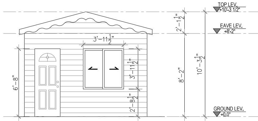
1 FRONT ELEVATION Scale 1"=1/4"
