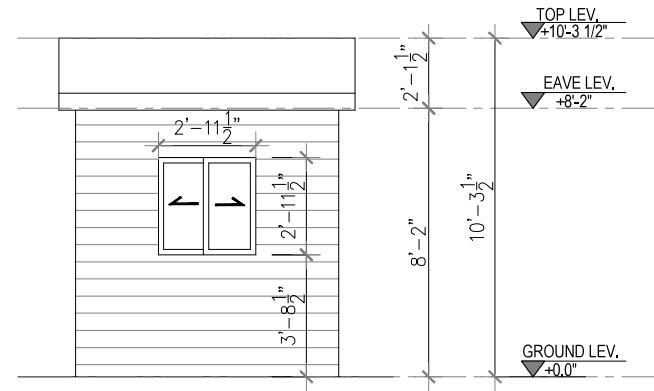
3 RIGHT SIDE ELEVATION Scale 1"=1/4"
