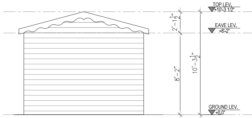
2 REAR ELEVATION Scale 1"=1/4"
