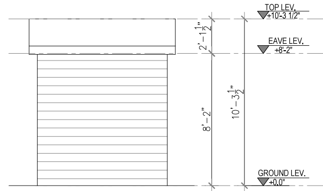
4 LEFT SIDE ELEVATION Scale 1"=1/4"
