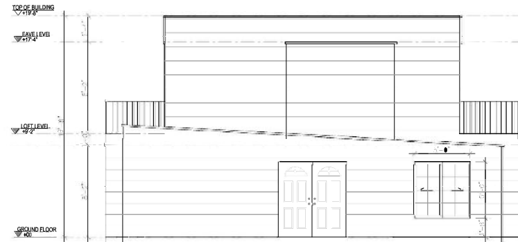
4 RIGHT SIDE ELEVATION Scale 1"=1/8"
