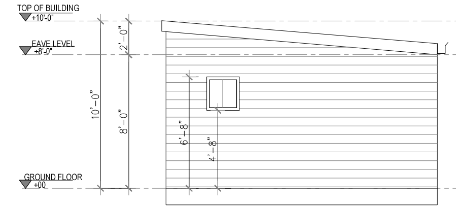
4 LEFT ELEVATION Scale 1=1/4"
