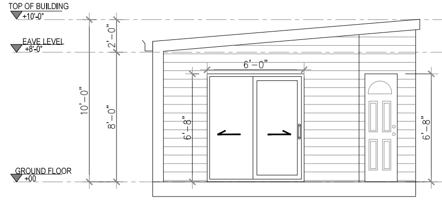
3 RIGHT ELEVATION Scale 1=1/4"
