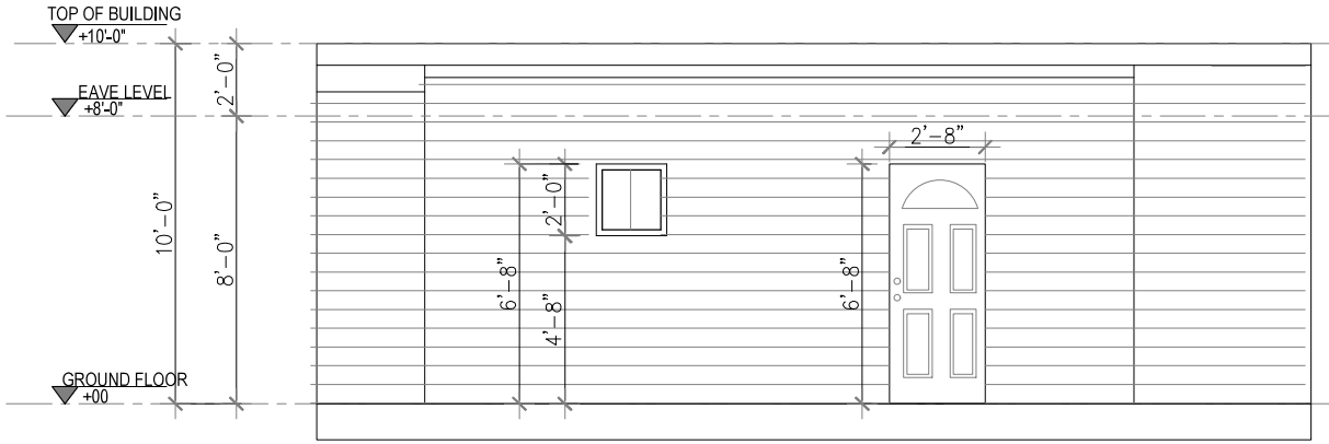
1 FRONT ELEVATION Scale 1=1/4"
