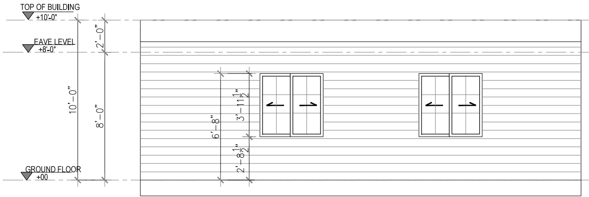
2 REAR ELEVATION Scale 1=1/4"
