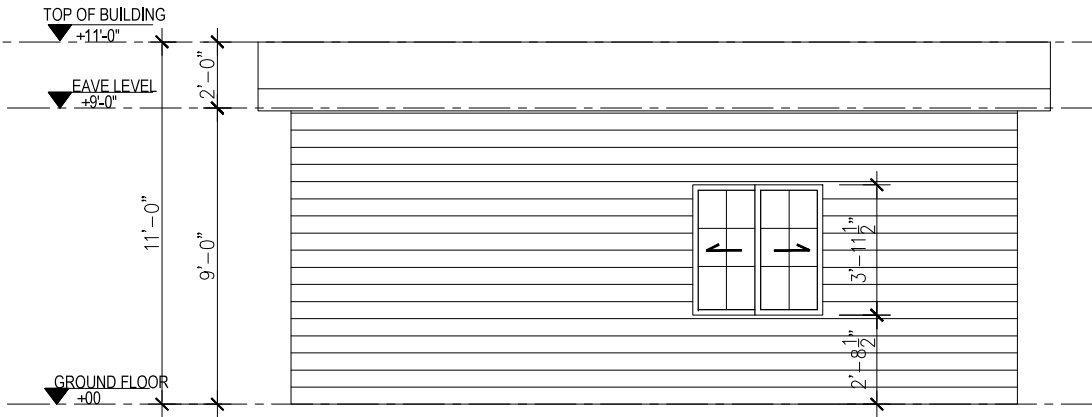
2 REAR ELEVATION Scale 1"=1/4"
