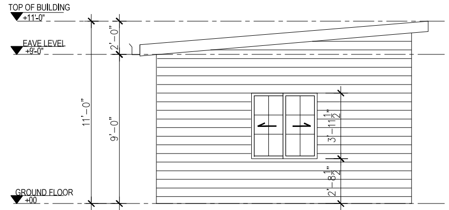
4 LEFT SIDE ELEVATION Scale 1"=1/4"
