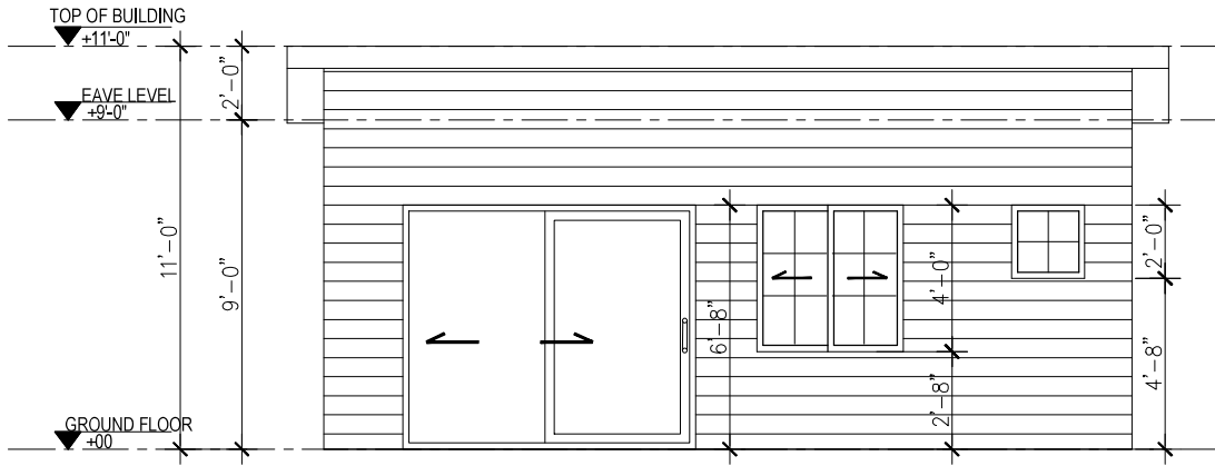
1 FRONT ELEVATION Scale 1"=1/4"
