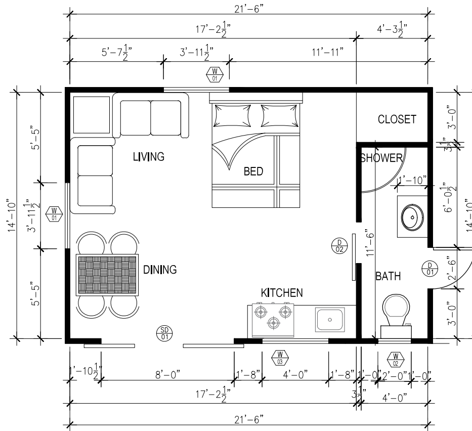
1 GROUND FLOOR PLAN Scale 1"=1/4"
