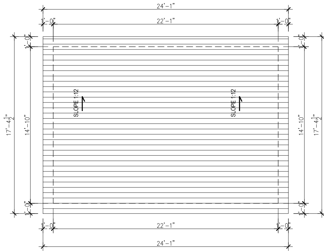
2 ROOF FLOOR PLAN Scale 1"=1/4"
