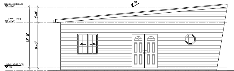
3 RIGHT SIDE ELEVATION Scale 1"=1/8"
