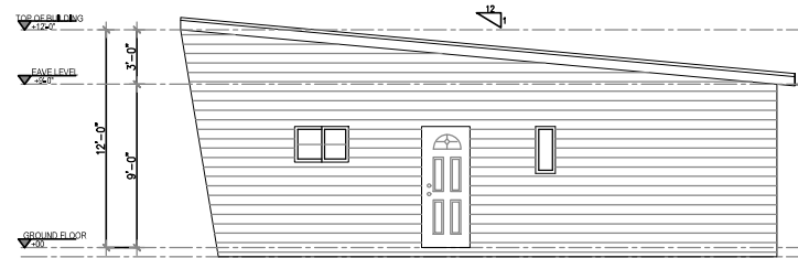
4 LEFT SIDE ELEVATION Scale 1"=1/8"
