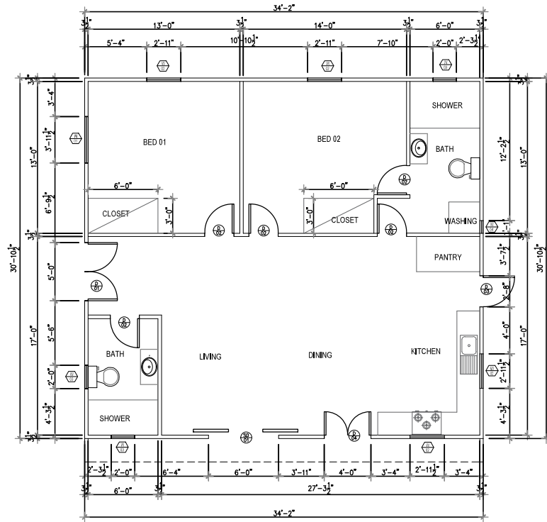
1 GROUND FLOOR PLAN Scale: 1"=1/8"
