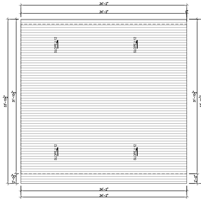
2 ROOF FLOOR PLAN Scale: 1"=1/8"
