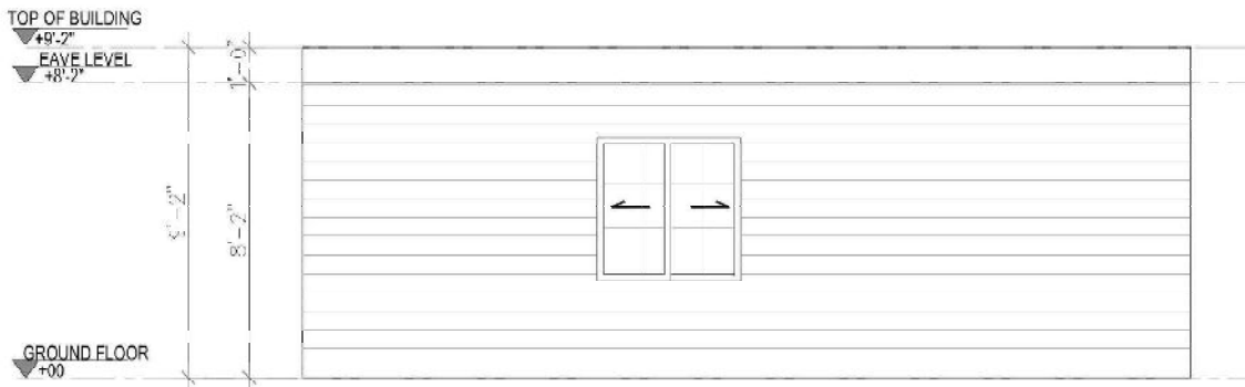
2 REAR ELEVATION Scale 1'=1/4"
