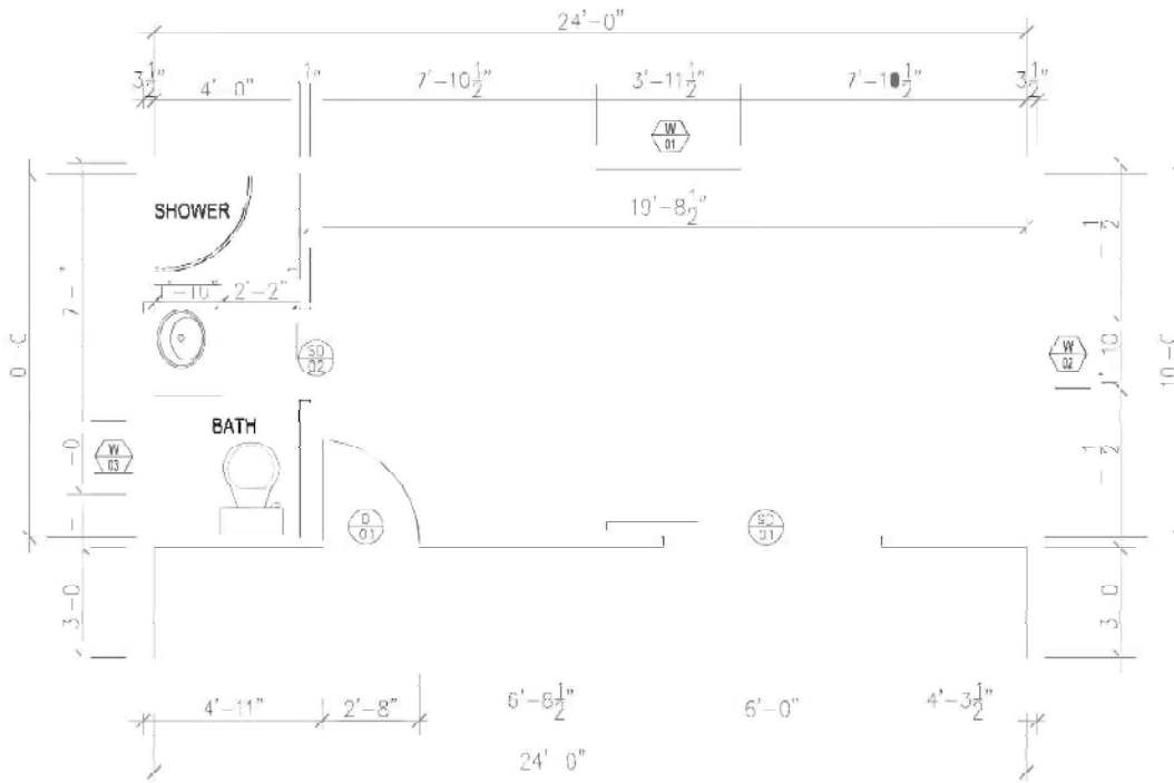
1 GROUND FLOOR PLAN Scale 1'=1/4"
