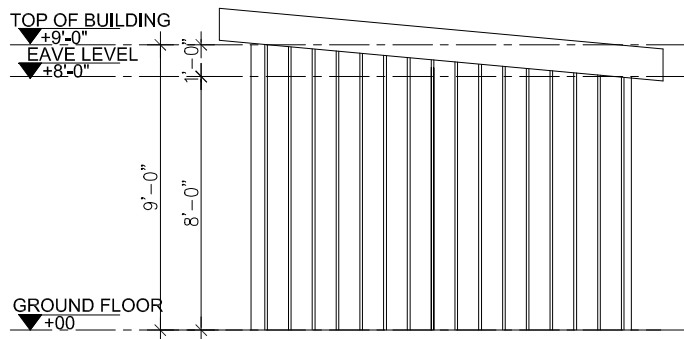
1 REAR ELEVATION Scale 1'=1/4"
